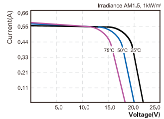
I-V Curves of PV module ECS-10P-36 at various cell temperatures
