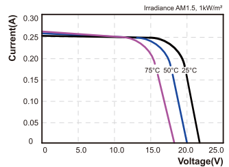
I-V Curves of PV module ECS-5M-36 at various cell temperatures
